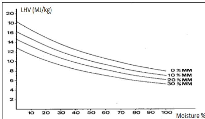
Fig.7: Evolution of lignocellulosic materials low heating value LHV according to the moisture concentration and of minerals matter [26]
