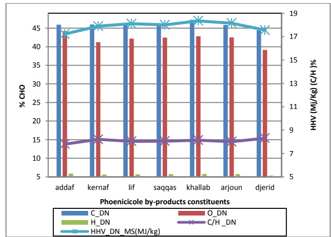
Fig.9: Comparison between elemental composition and calorific value HHV of cultivar DN
