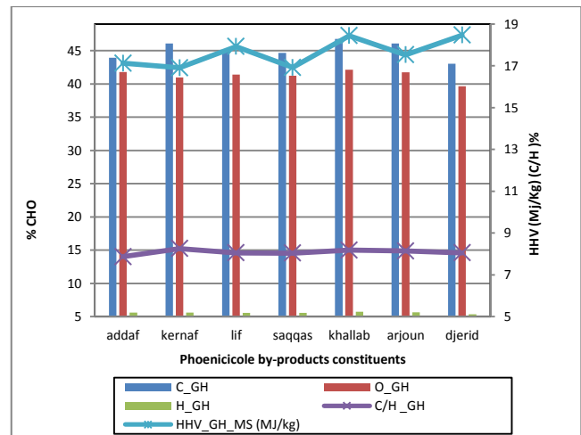
Fig.10: Comparison between elemental composition and calorific value HHV of cultivar GH
