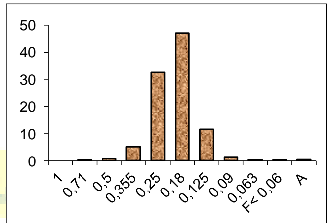
Figure 3. Histogram representation of granulometric analysis of Taghit sand.
