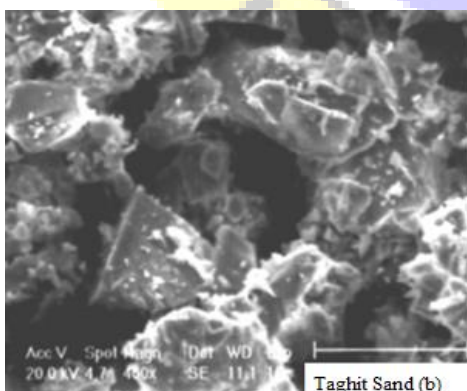
Figure 6. The Scanning electron Micrograph of Taghit sand ( higher magnitude)
