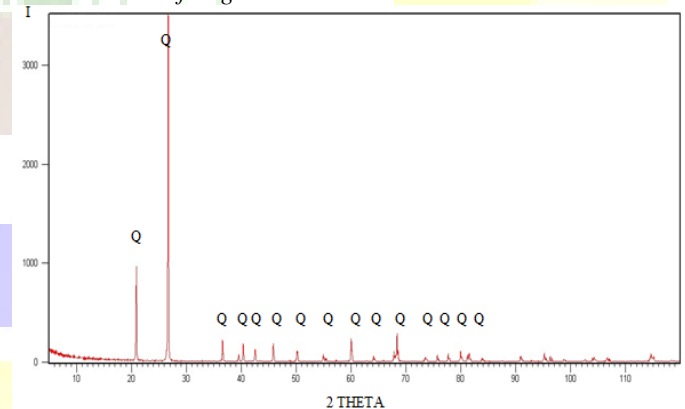
Figure 4. The XRD spectrum of Taghit sand.
